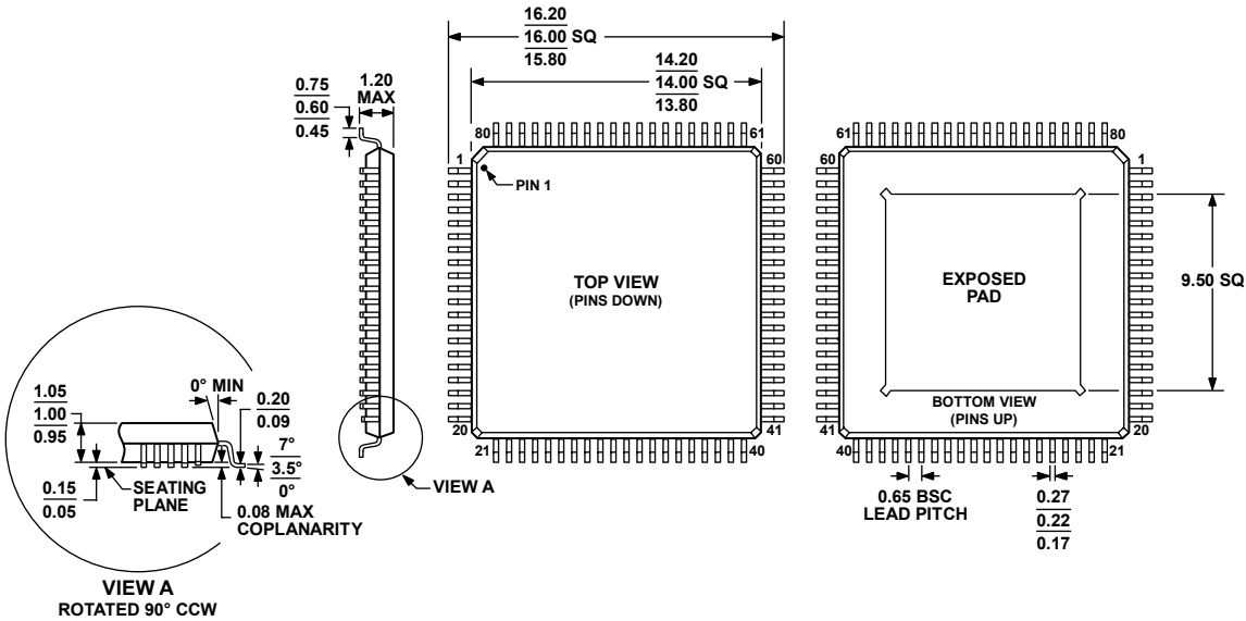
COMPLIANT TO JEDEC STANDARDS MS-026-AEC-HD Figure 71. 80-Lead Thin Quad Flat Package, Exposed Pad [TQFP_EP] (SV-80-4) Dimensions shown in millimeters
