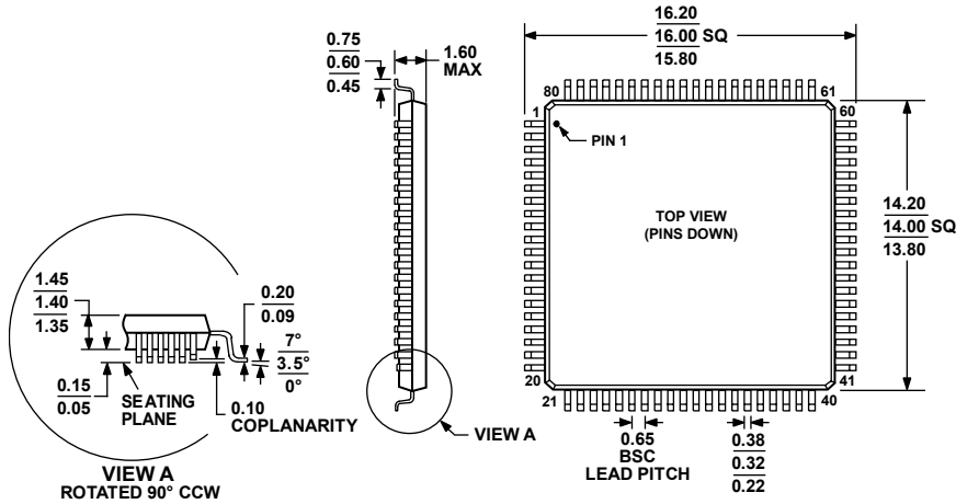
COMPLIANT TO JEDEC STANDARDS MS-026-BEC Figure 72. 80-Lead Low Profile Quad Flat Package [LQFP] (ST-80-2) Dimensions shown in millimeters
